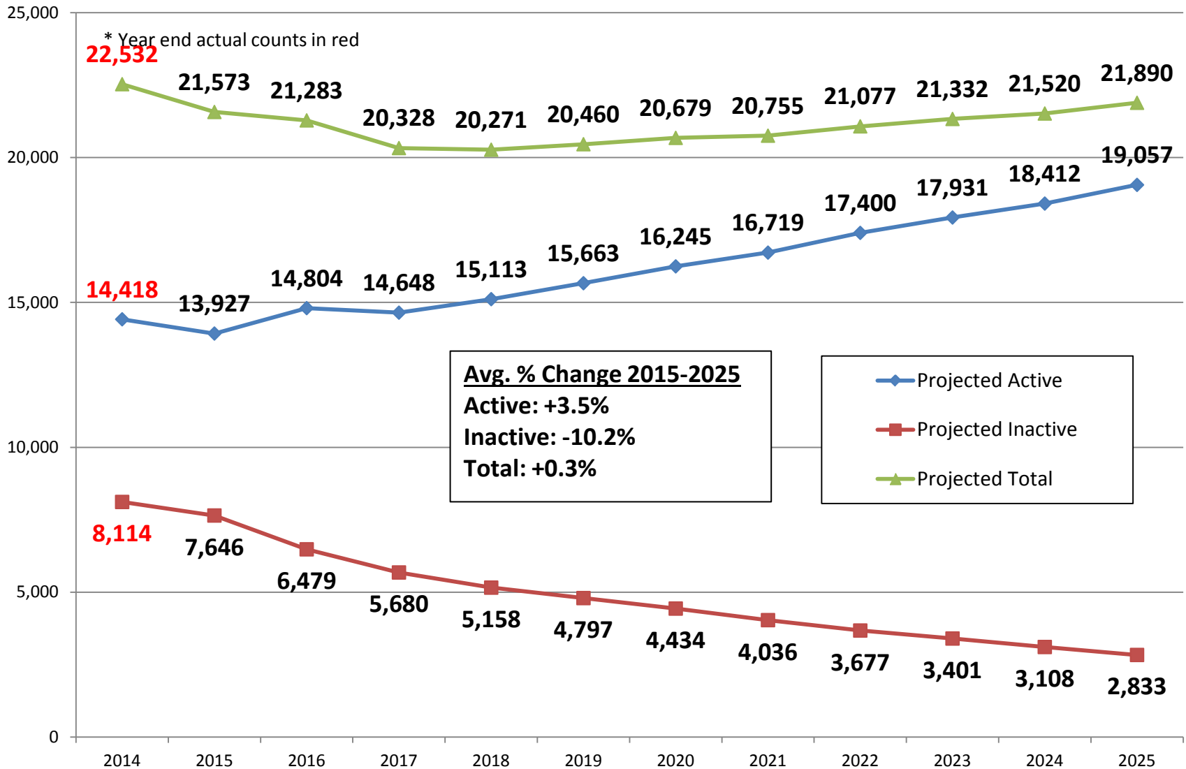
Figure 13: Parole Projections
